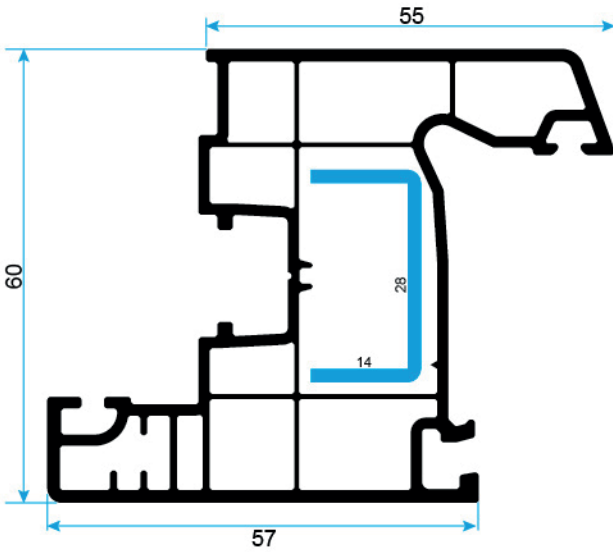
PENCERE KANAT PROFİLİ SASH PROFILE
