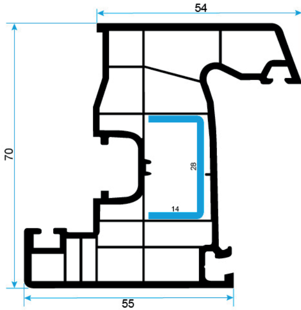
PENCERE KANAT PROFİLİ SASH PROFILE
