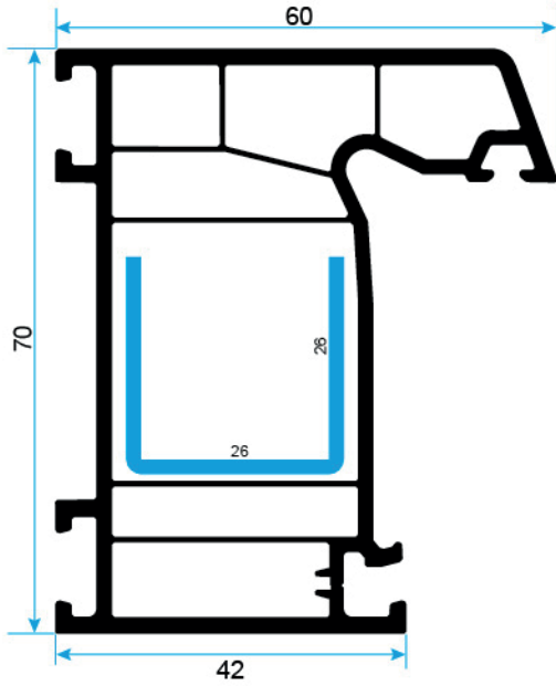
KASA PROFİLİ FRAME PROFILE
