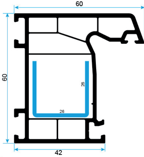
KASA PROFİLİ FRAME PROFILE
