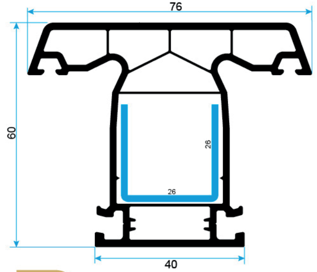
ORTA KAYIT PROFİLİ MULLION PROFILE
