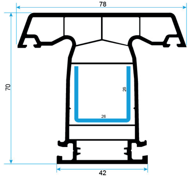
ORTA KAYIT PROFİLİ MULLION PROFILE
